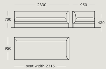
Module 6 3.5 seater, right arm Back cushions not included
