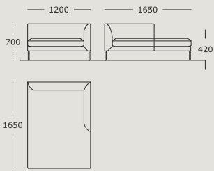
Module 16 2 seater, terminal right arm - wide Back cushions not included
