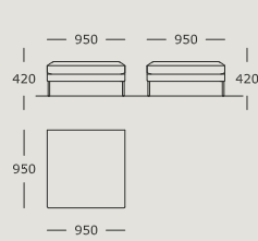
Module 23 Stool Back cushions not included
