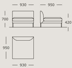
Module 22 Center Back cushions not included
