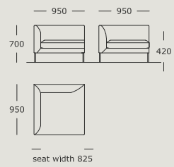
Module 21 Corner Back cushions not included
