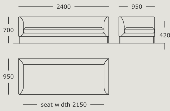
Module 1 3.5 seater Back cushions not included
