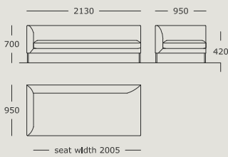
Module 7 3 seater, left arm Back cushions not included
