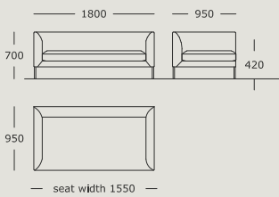
Module 4 2 seater Back cushions not included
