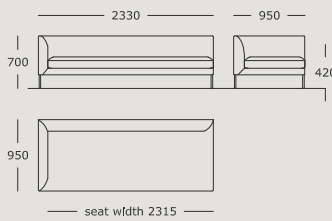
Module 5 3.5 seater, left arm Back cushions not included
