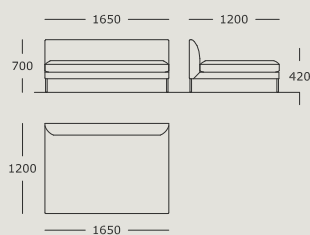
Module 13 2 seater, chaise no arms - wide Back cushions not included
